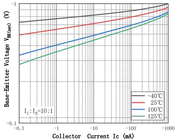
Fig.4 - Base-Emittor Voltage
